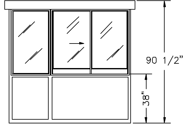
ELEVATION C
