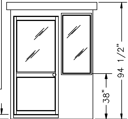
ELEVATION C
